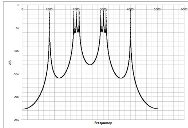
FIGURE 6. Minimum Variance Spectrum
